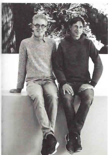
122_CONVERSATION
